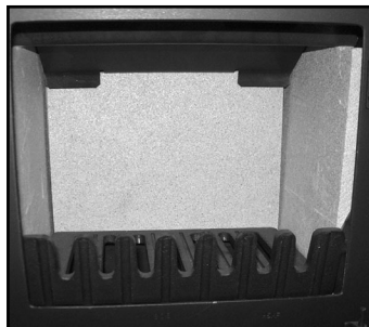
Fig. 3 Liners, throat plate and grate in the Willow.
