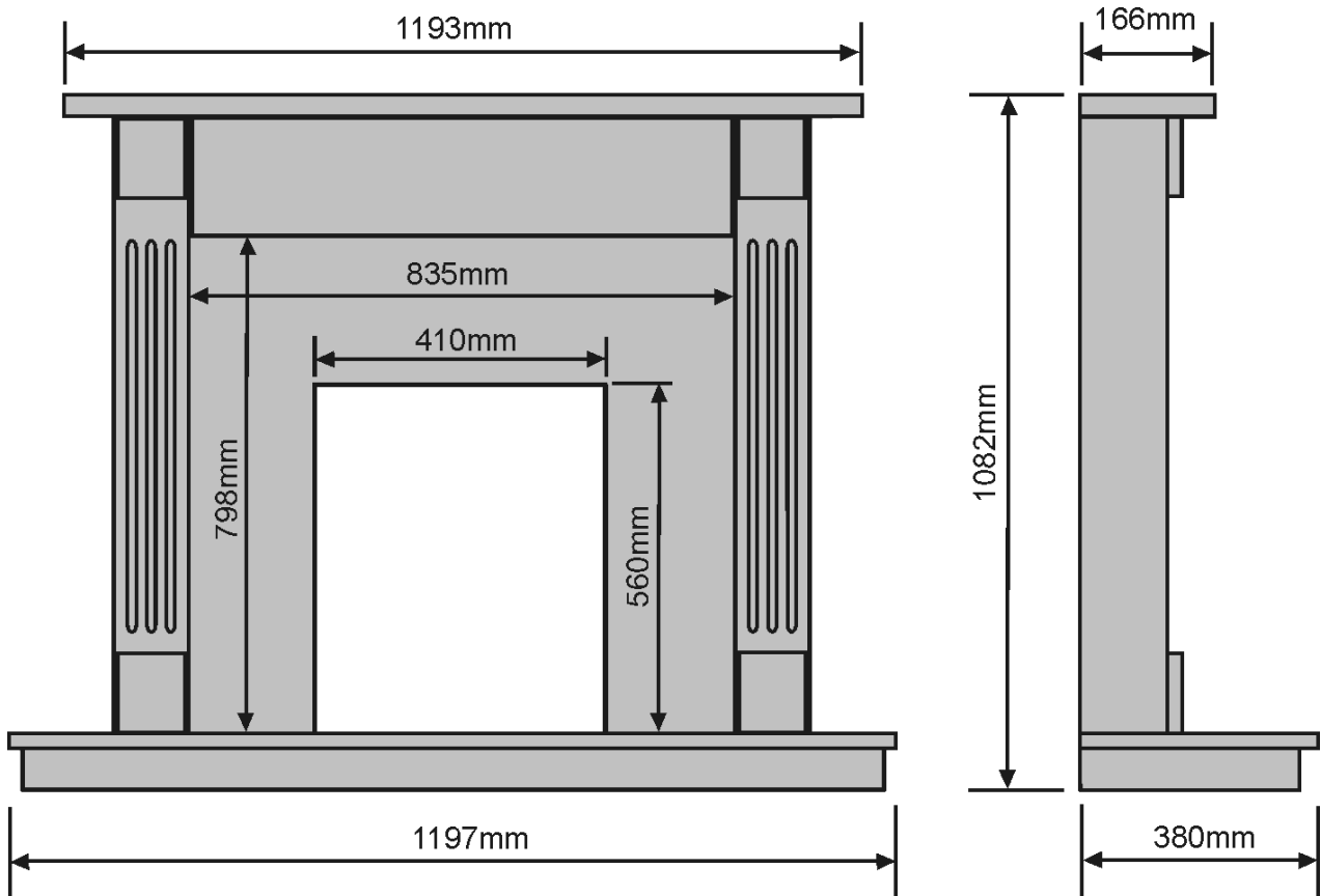
Figure 1. Dimensions
