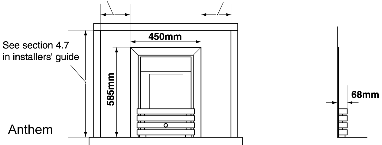
Figure 1. Appliance dimensions
