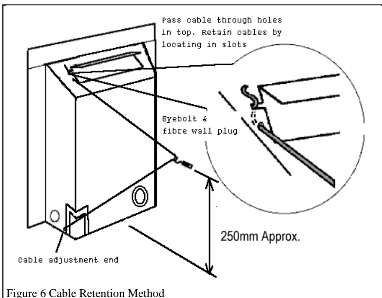
Figure 6 Cable Retention Method
