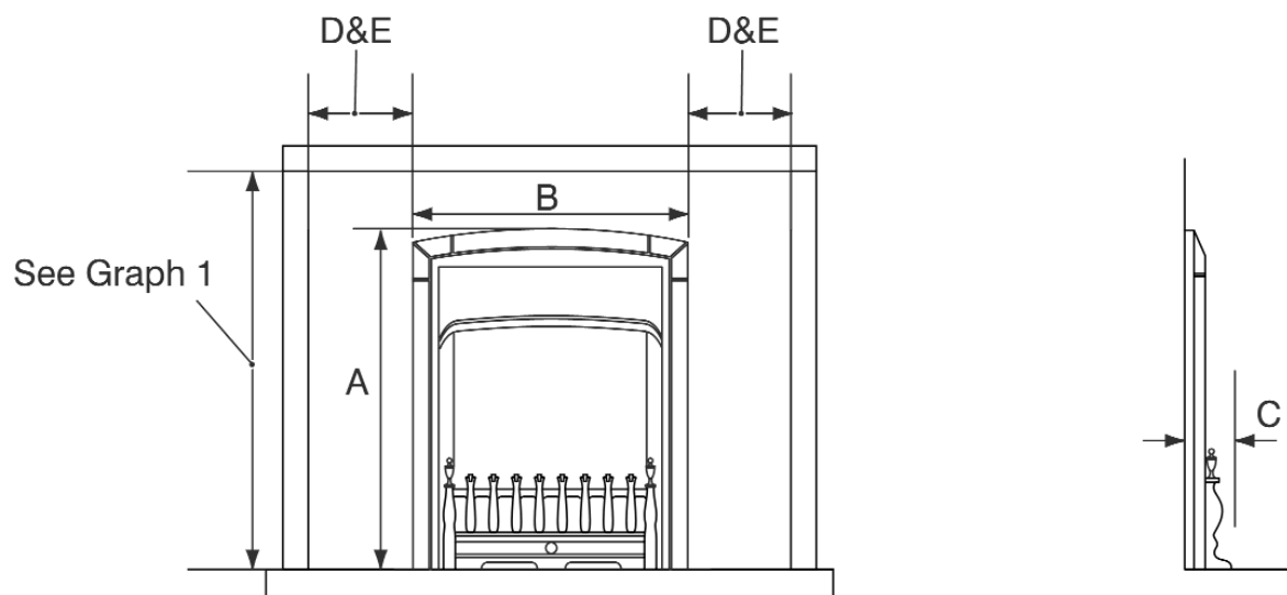
Figure 1. Appliance dimensions and clearances - SEE TABLE ON NEXT PAGE (Fascia may differ from that shown)
