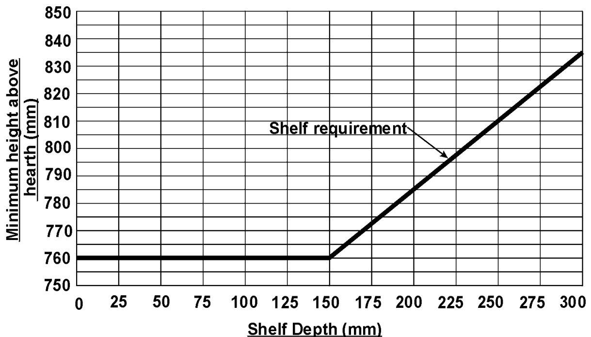
Graph 1. Combustible shelf clearances.
