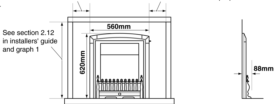
Figure 1. Appliance dimensions
