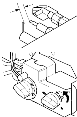
Figure 4 Ignition check
