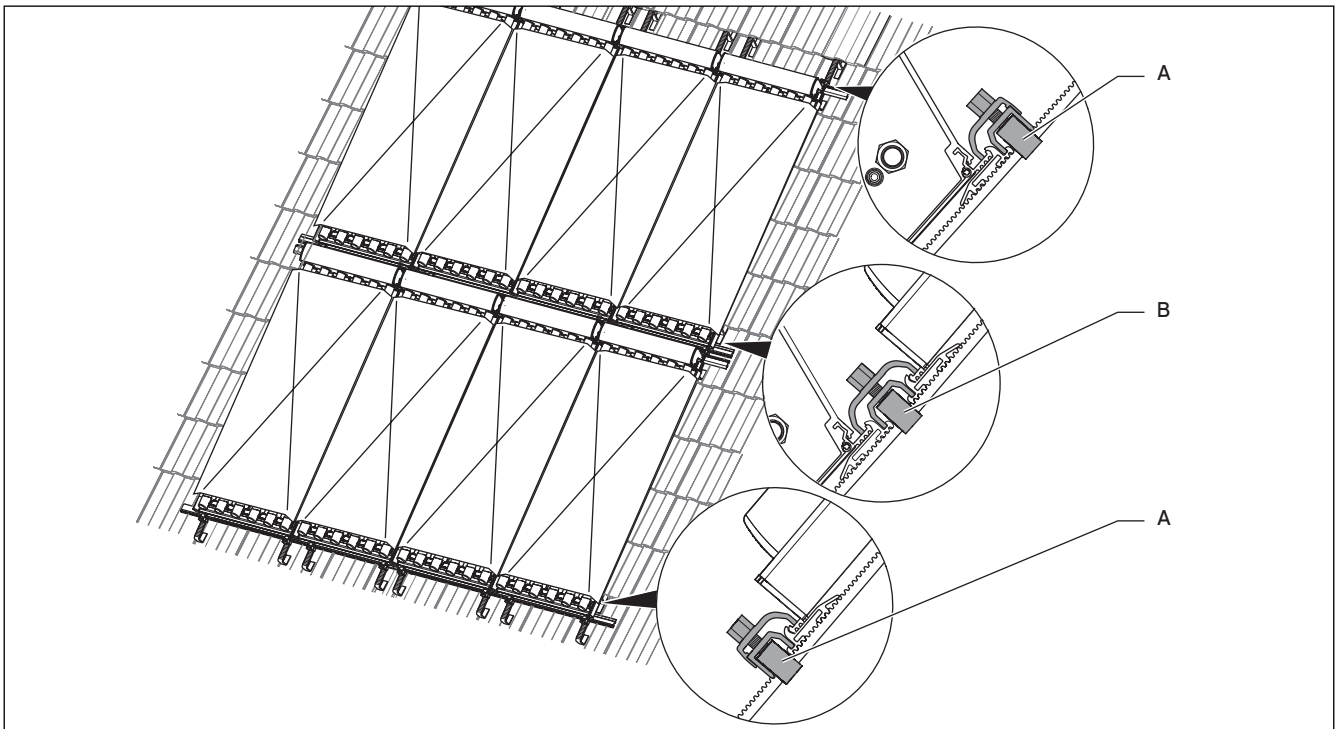
Fig. 4.4 Installation kit for 2-row on-roof mounting (here: VTK 570/2)
