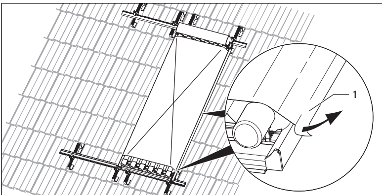
Fig. 5.13 Peeling the film from the edges of the collector
