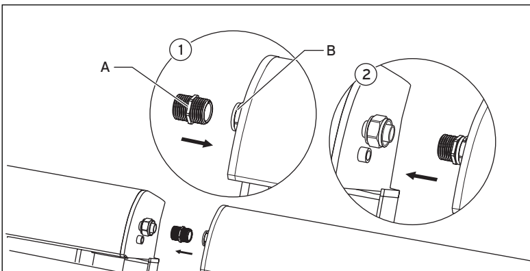
Fig. 6.13 Joining the collectors
