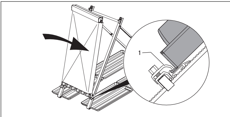
Fig. 6.9 Hooking the collector
