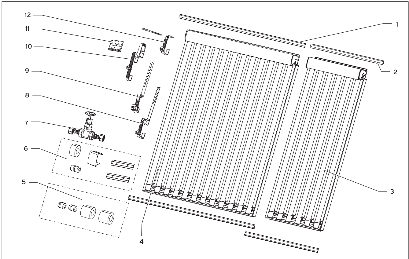
Fig. 4.1 On-roof mounting kit
