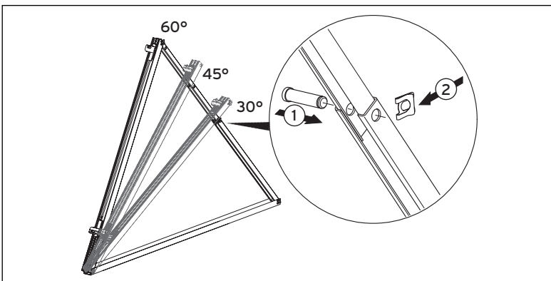
Fig. 6.3 Frame assembly
