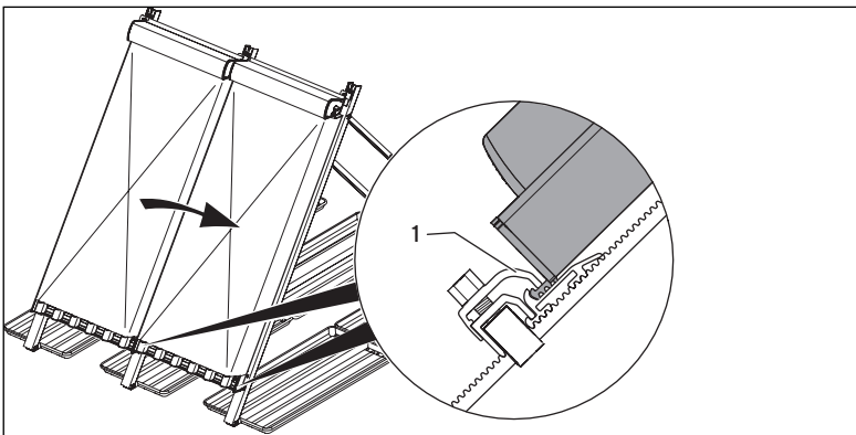
Fig. 6.12 Mounting other collectors
