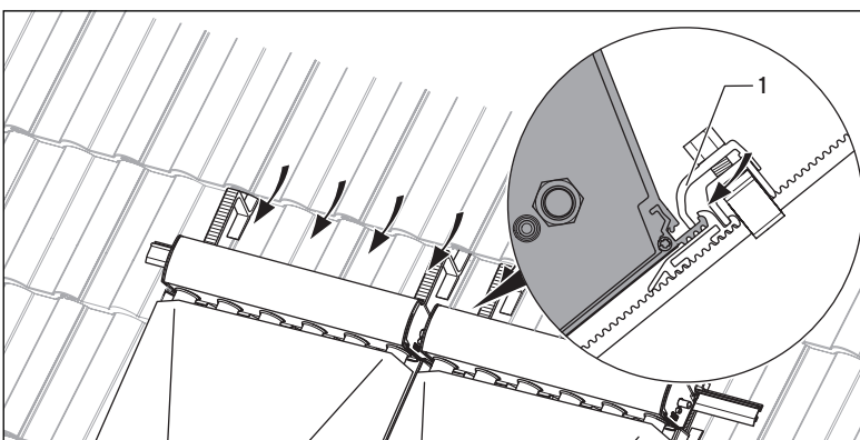
Fig. 5.18 Positioning the upper mounting rail
