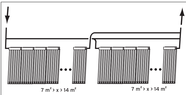
Fig. 4.8 Parallel connection (here VTK 570/2)
