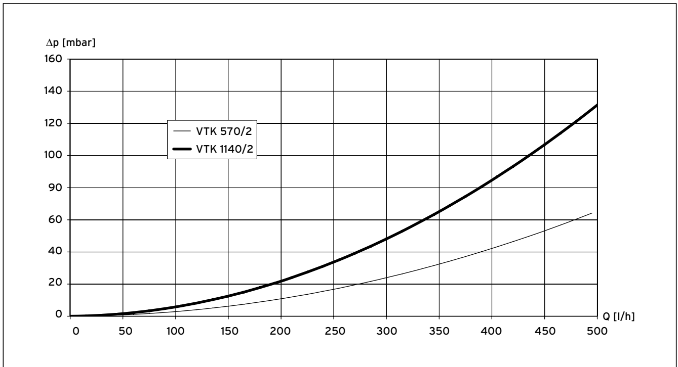
Fig. 10.5 Pressure loss graph
