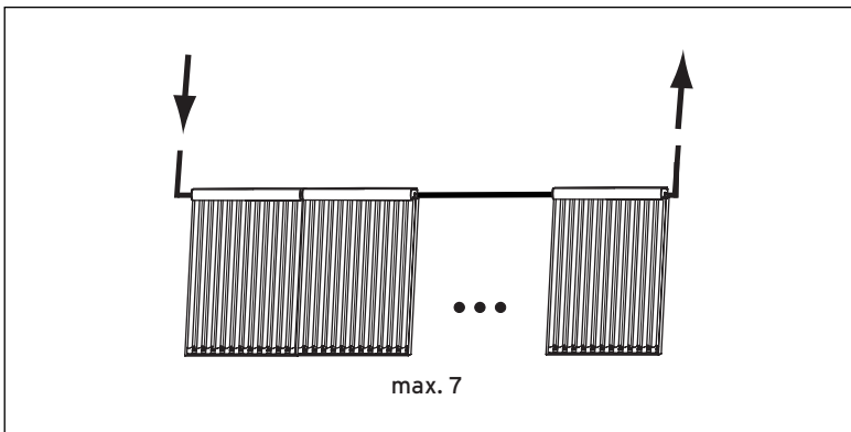
Fig. 4.7 Series connection VTK 1140/2
