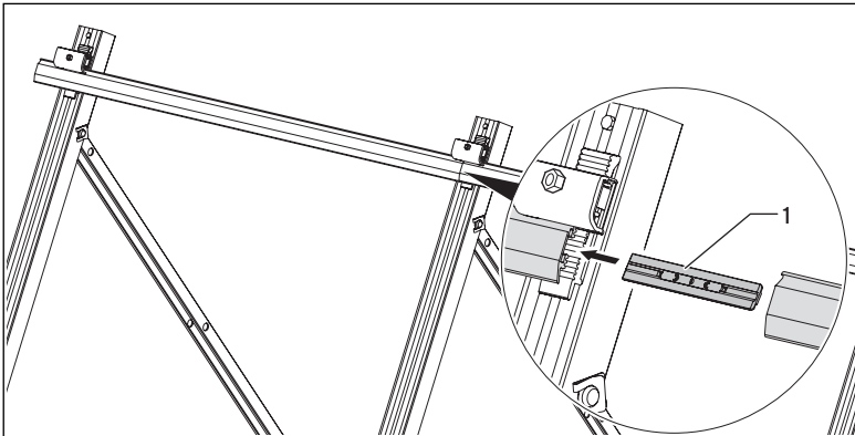
Fig. 6.8 Joining the mounting rails
