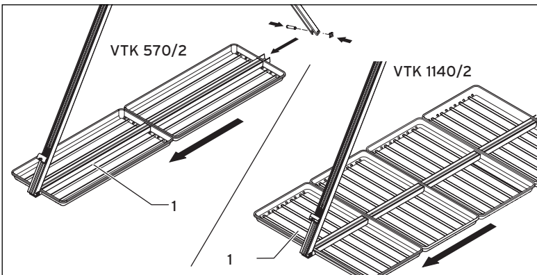
Fig. 6.2 Mounting the gravel trays
