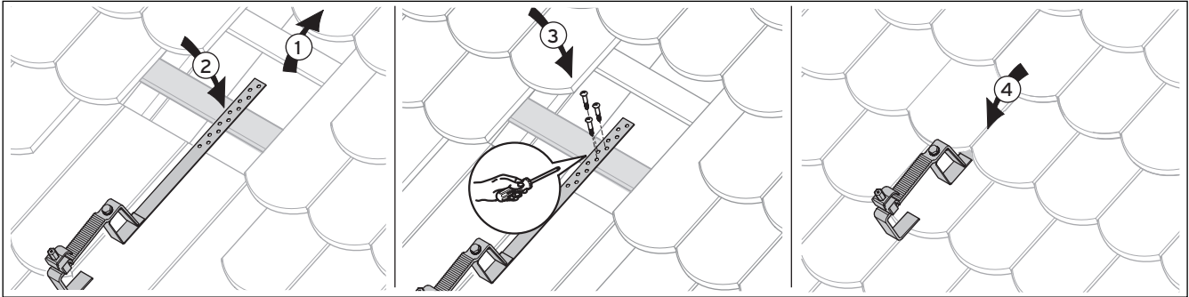
Fig. 5.6 Fixing the bracket type S
