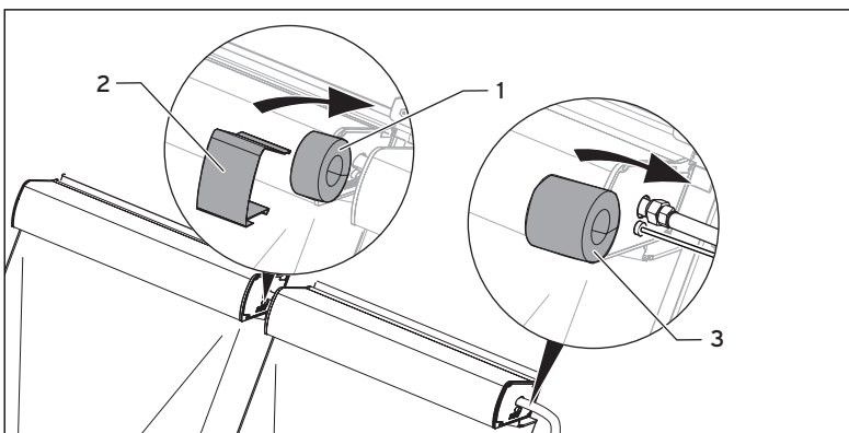
Fig. 5.22 Insulating the hydraulic connections
