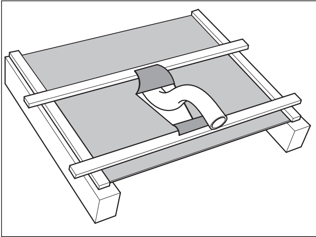
Fig 4.11 Passing the pipe through the sarking membrane
