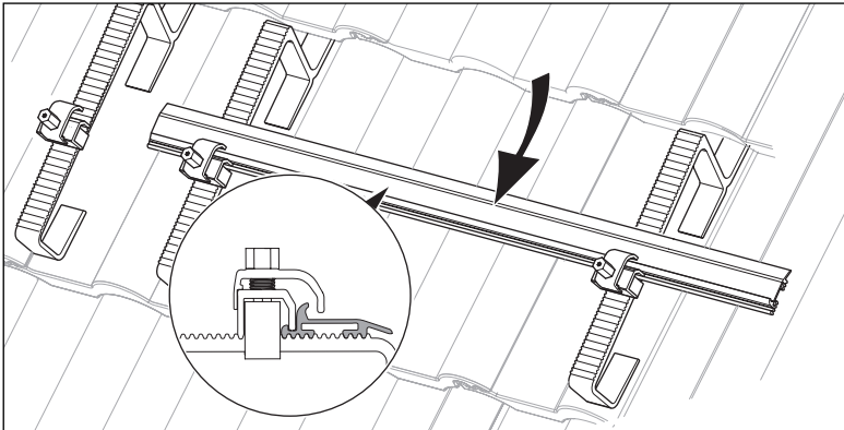
Fig. 5.9 Fixing the mounting rails
