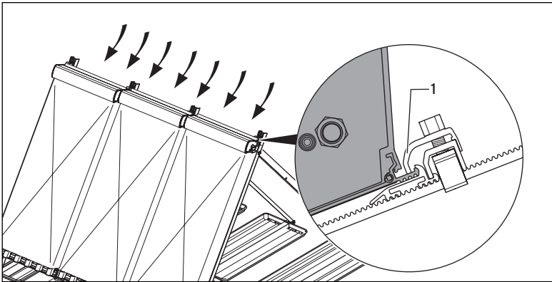
Fig. 6.15 Positioning the upper mounting rail
