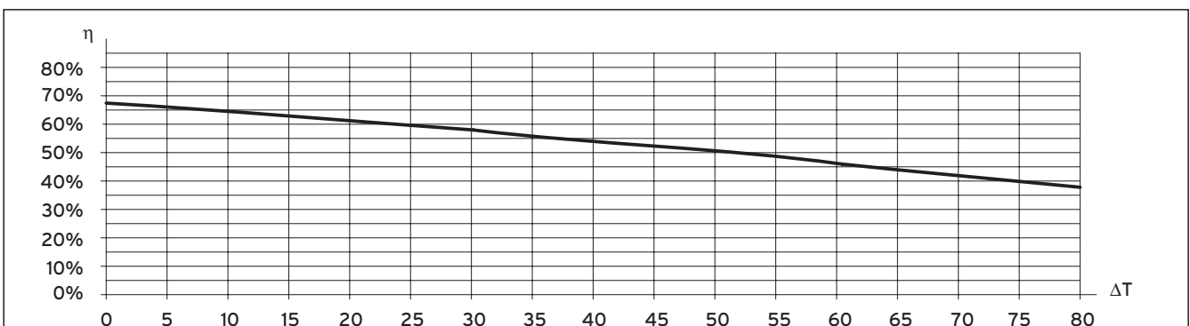
Fig. 10.3 Efficiency of the VTK 570/2 and the 1140/2 at an irradiance E_g of 300 \text{ W/m}^2
