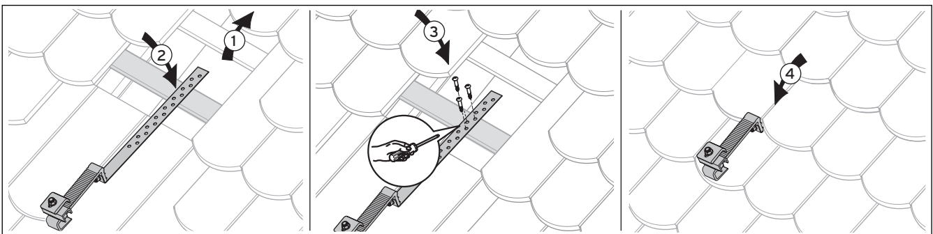
Fig. 5.7 Fixing the bracket type S flat
