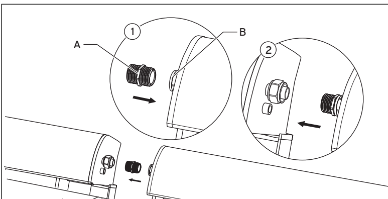
Fig. 5.16 Joining the collectors
