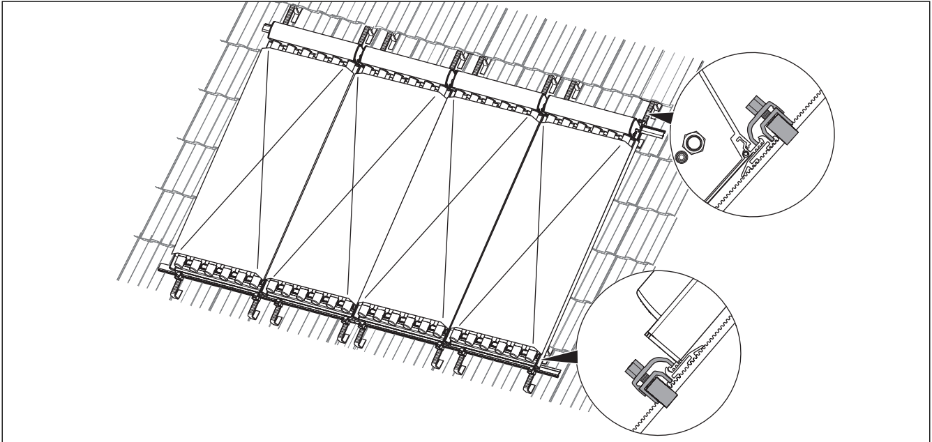
Fig. 4.3 Installation kit for single row on-roof mounting (here: VTK 570/2)
