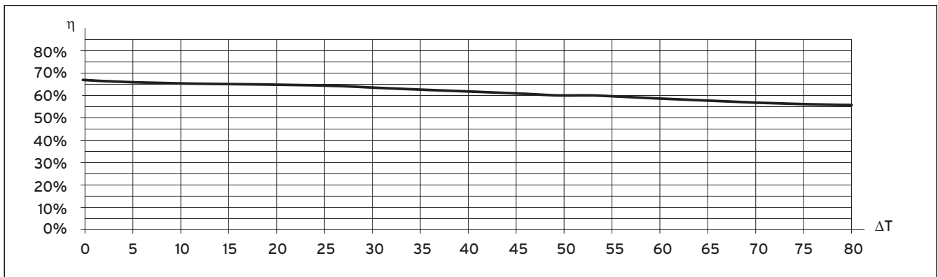
Fig. 10.4 Efficiency of the VTK 570/2 and the 1140/2 at an irradiance E_g of 800 \text{ W/m}^2
