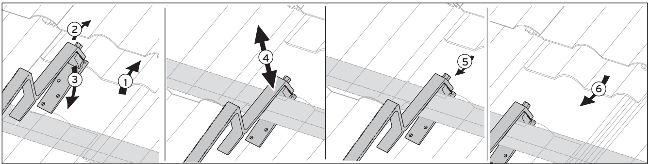
Fig. 5.5 Fixing to the roof batten
