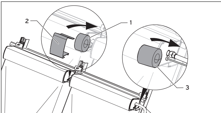
Fig. 6.17 Insulating the hydraulic connections
