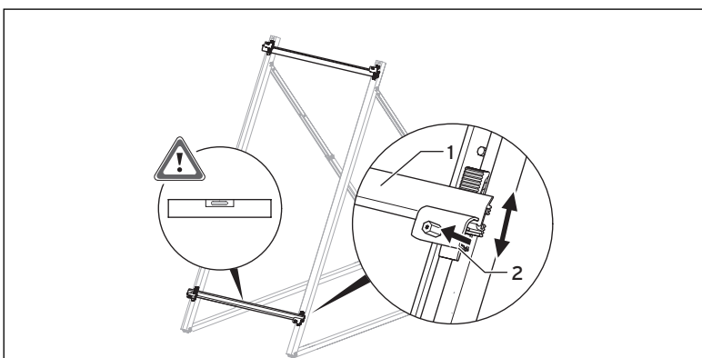
Fig. 6.6 Fixing and blocking the mounting rail
