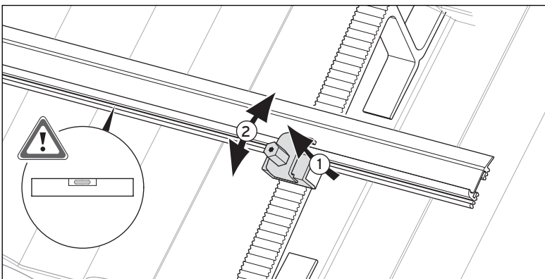
Fig. 5.11 Balancing the mounting rails
