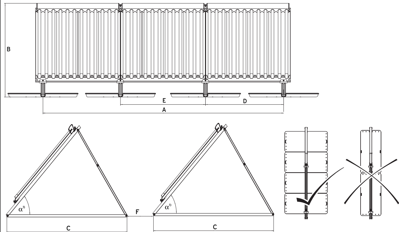
VTK 1140/2 [distances in mm]
