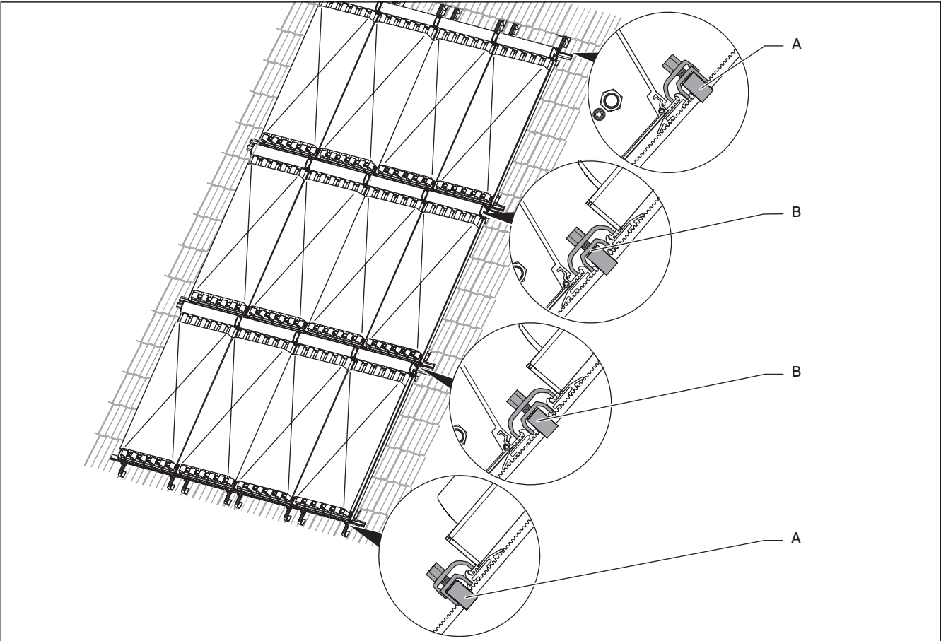
Fig. 4.5 Installation kit for 3-row on-roof mounting (here: VTK 570/2)
