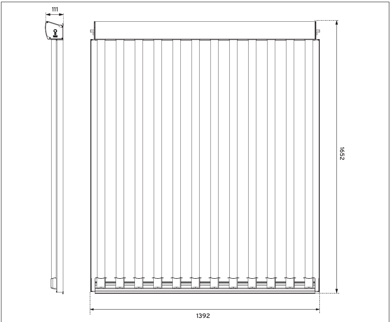
Fig. 10.2 Dimensional drawing VTK 1140/2
