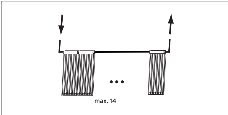
Fig. 4.6 Series connection VTK 570/2
