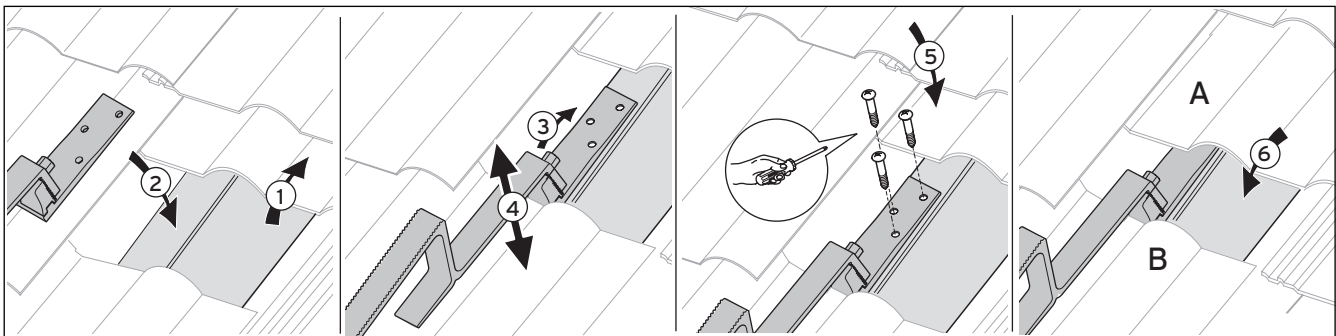
Fig. 5.4 Fixing to rafters
