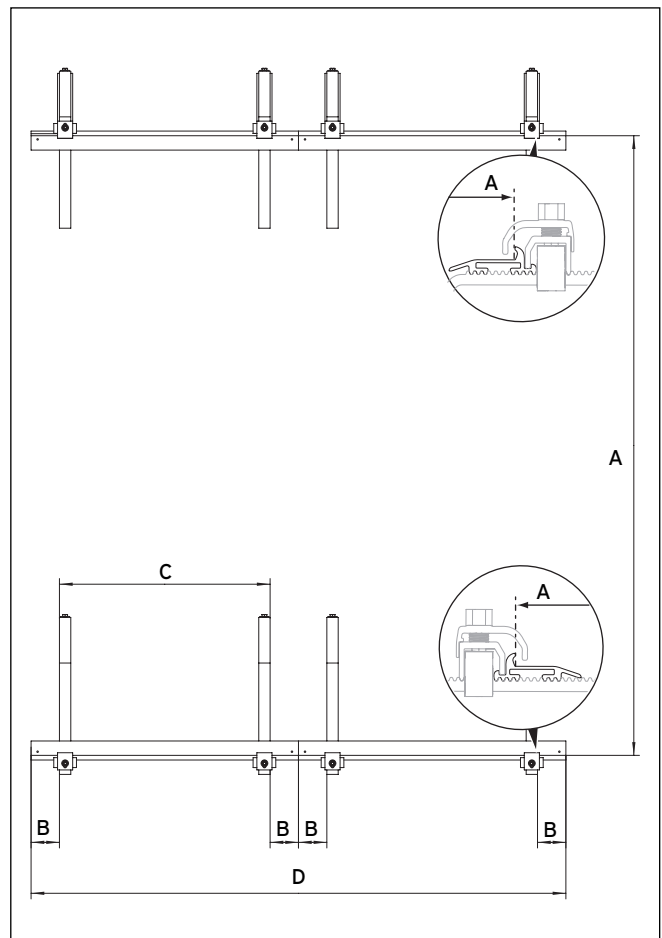
Fig. 5.1 Spacings when arranging collectors side-by-side
