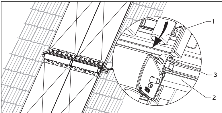
Fig. 5.20 Central mounting rail for 2 or 3 rows of collectors
