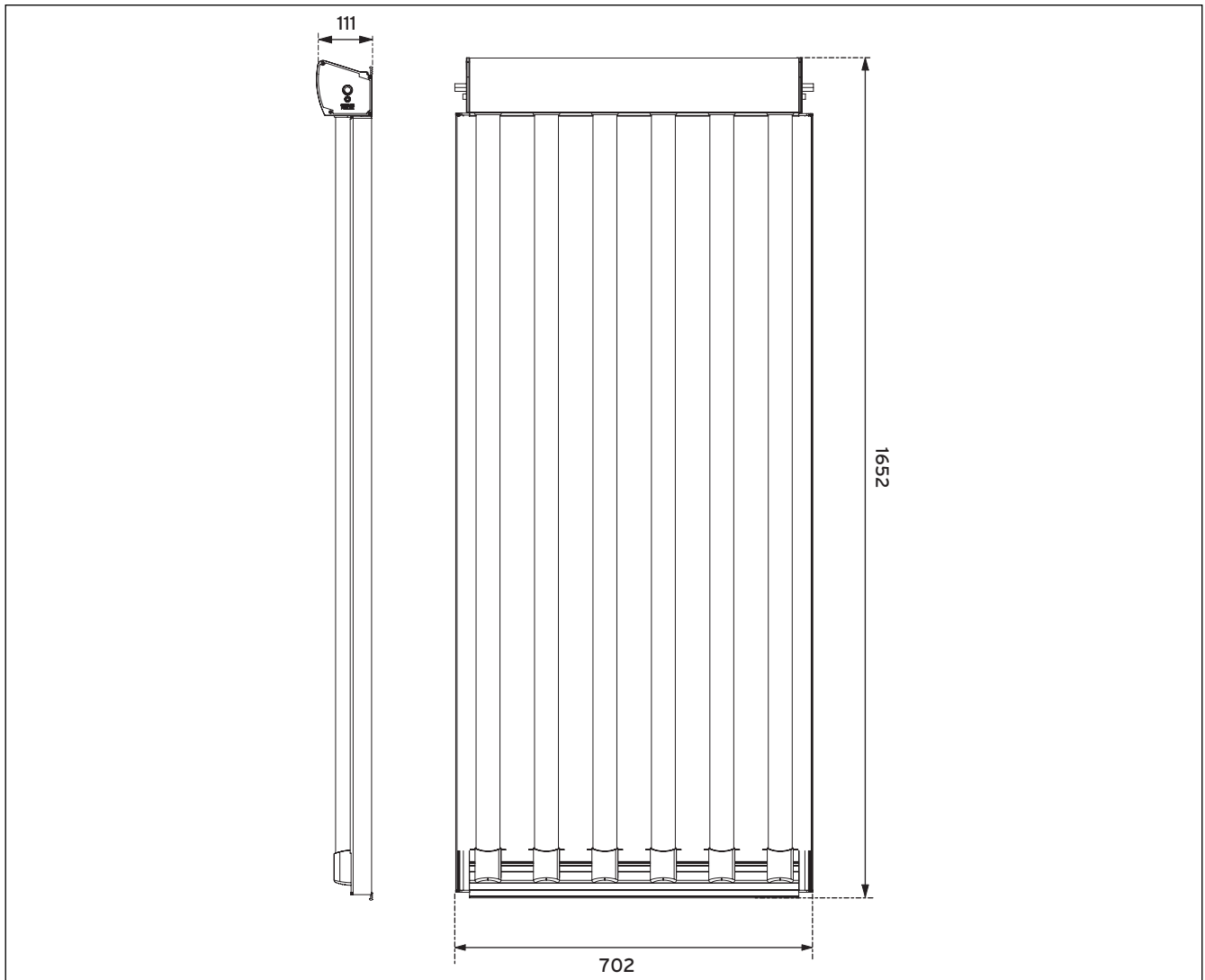
Fig. 10.1 Dimensional drawing VTK 570/2
