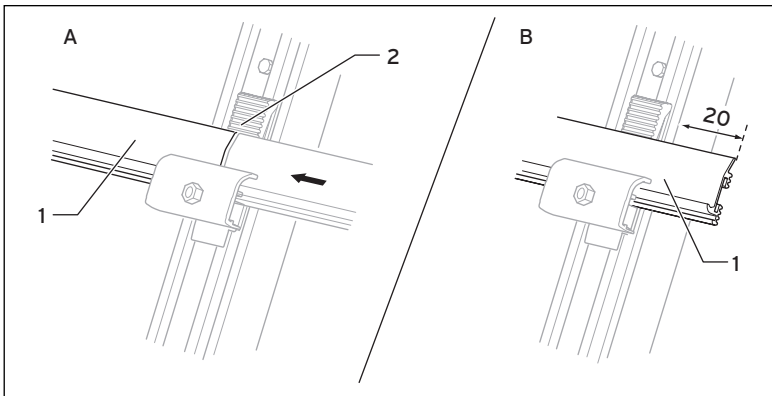
Fig. 6.7 Positioning the mounting rails
