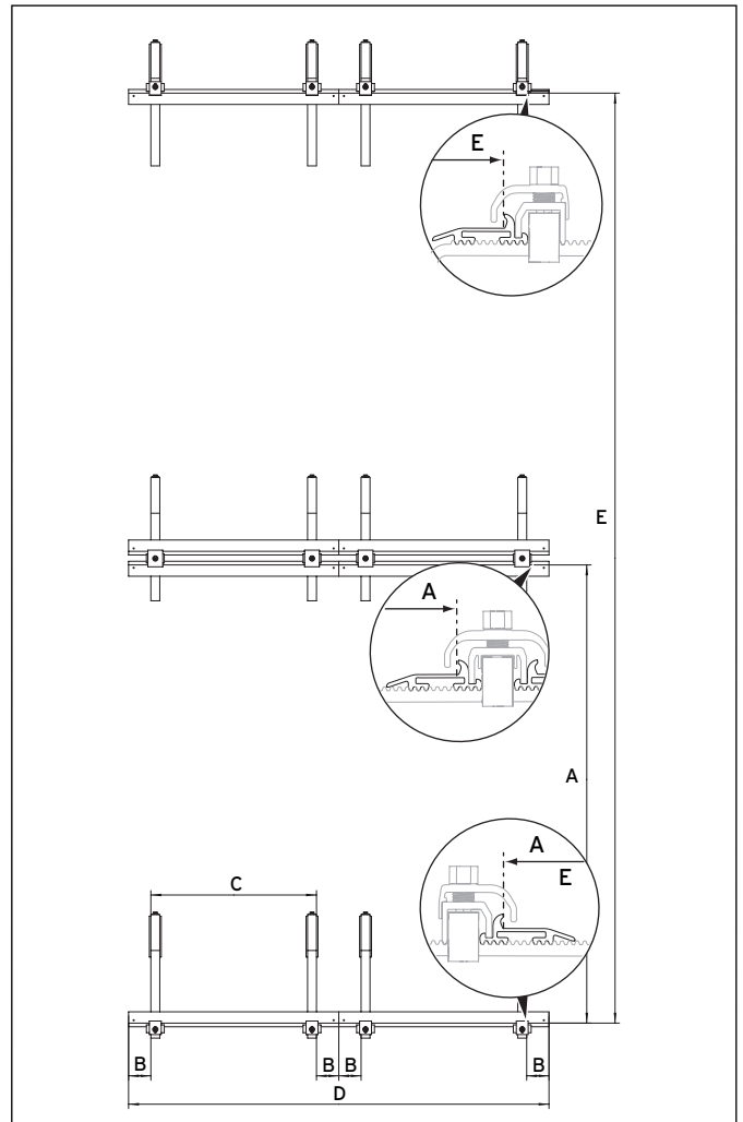
Fig. 5.2 Spacings when arranging collectors on top of each other
