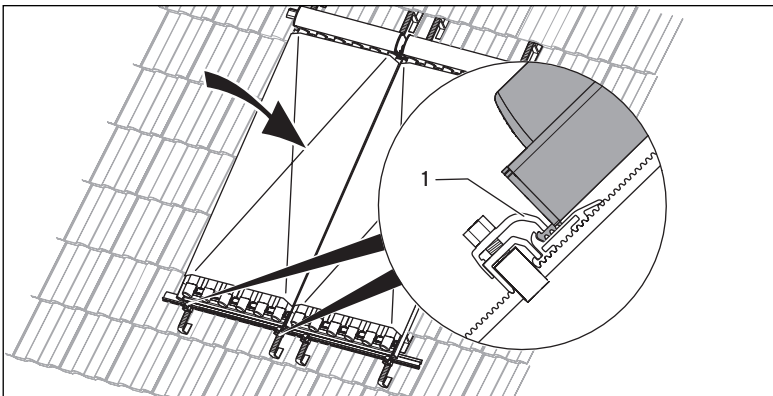
Fig. 5.15 Mounting other collectors
