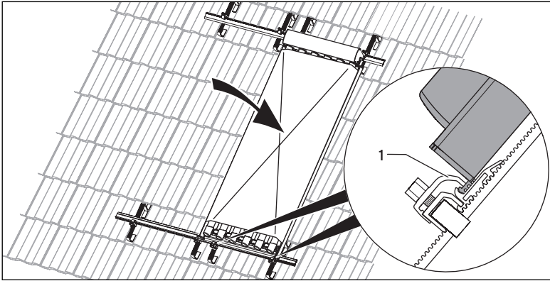
Fig. 5.12 Hooking the collector
