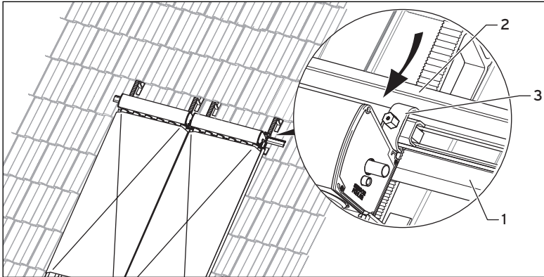
Fig. 5.19 Central mounting rail for 2 or 3 rows of collectors
