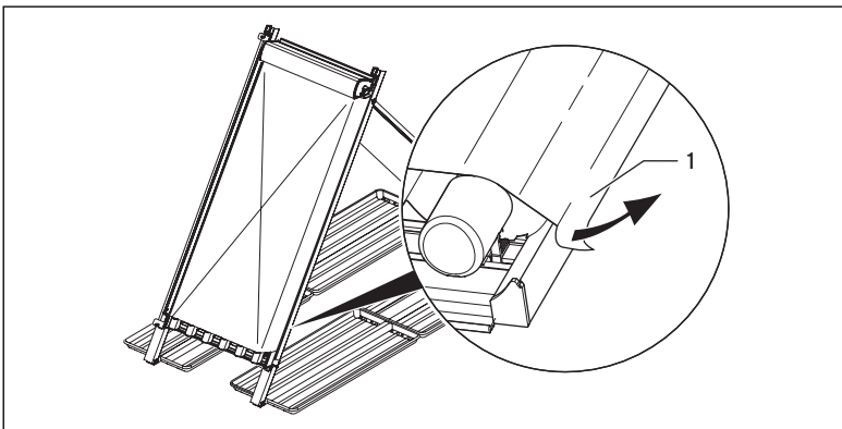
Fig. 6.10 Peeling the film from the edges of the collector
