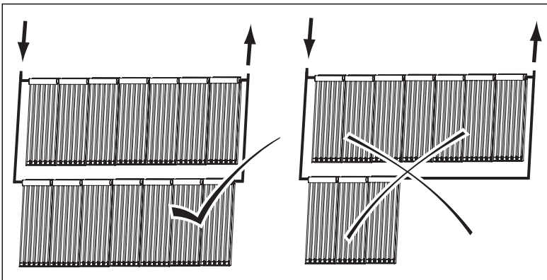
Fig. 4.9 Sizes of the individual arrays
