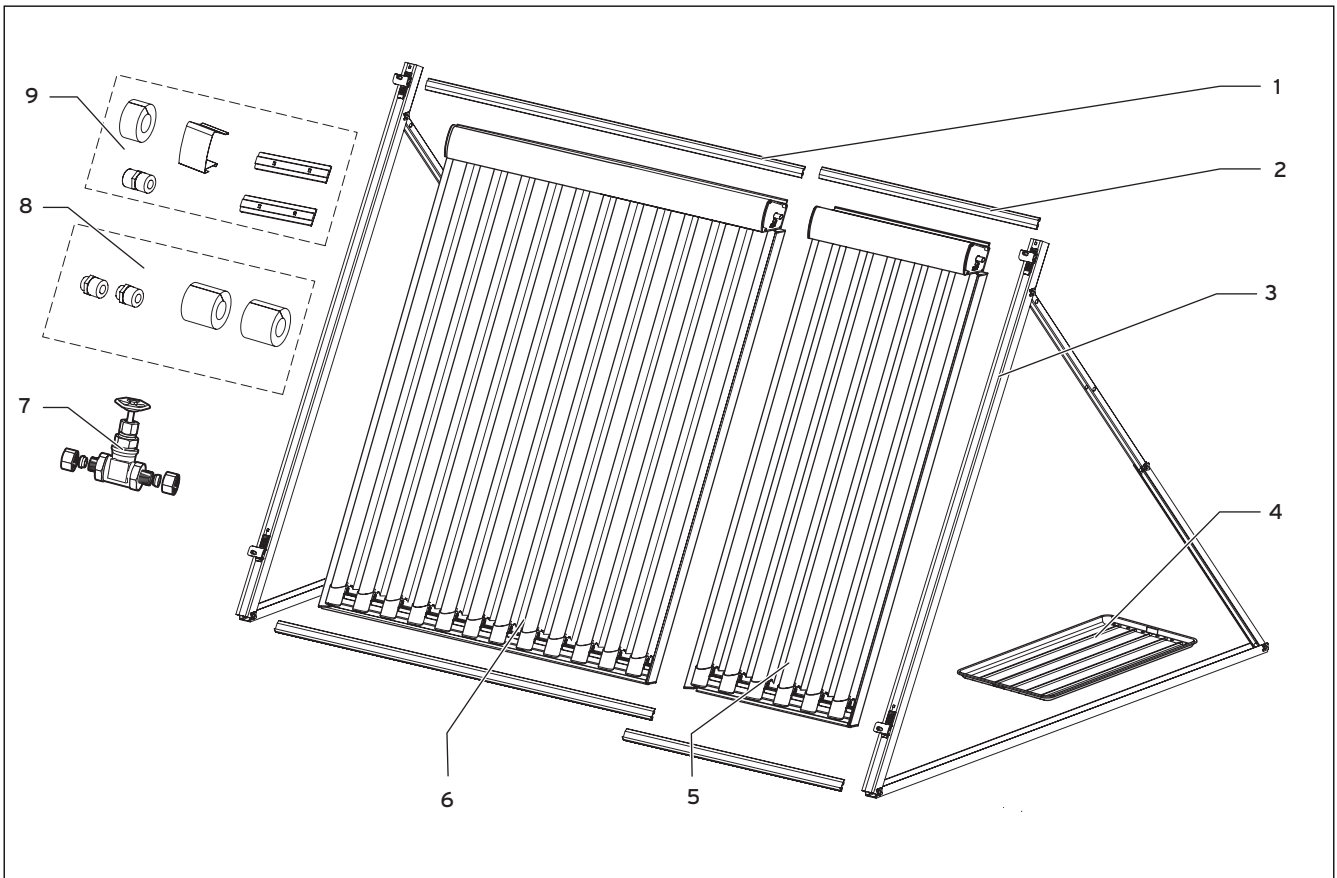
Fig. 4.2 Flat roof mounting kit
