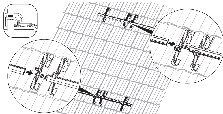
Fig. 5.10 Joining the mounting rails
