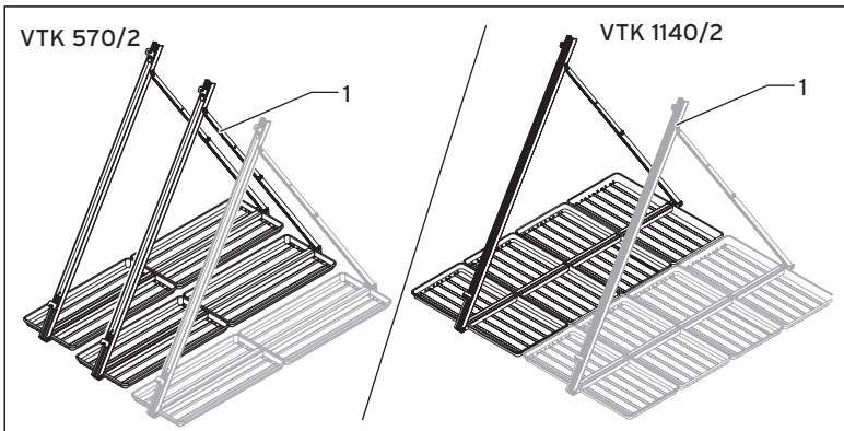
Fig. 6.4 Frames with gravel trays
