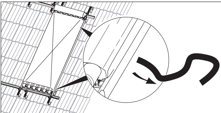
Fig. 5.14 Removing the carrying straps
