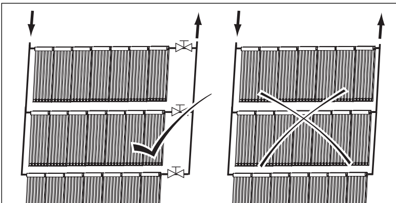
Fig. 4.10 Stop valve in the collector supply line
