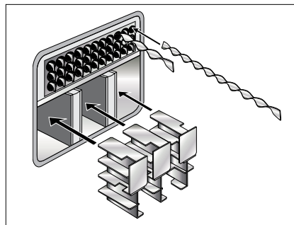
Baffle arrangement Grant Vortex 26-36 external module
