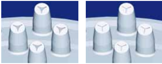
High flow rate: nozzles expand Low flow rate: nozzles contract
