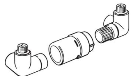
RTX sensor, RA-URX Right mounted and RLV-X left mounted.
