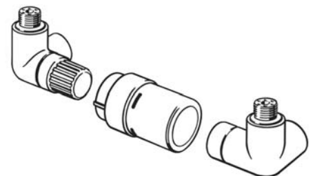
RTX sensor, RA-URX Left mounted and RLV-X Right mounted.
