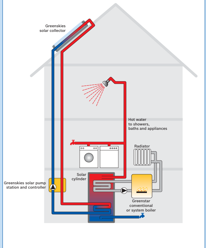
A typical solar system layout
