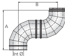
Offsets for Double 90° Bend
