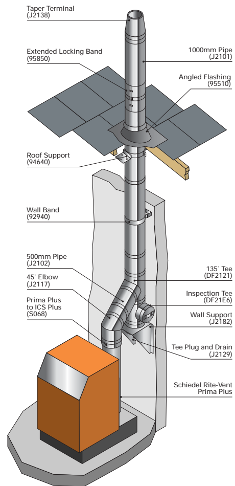
Fig.1 Distance to Combustibles from outer case of chimney
