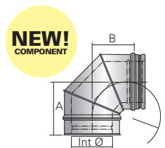
87° Bend ICS J21F3
