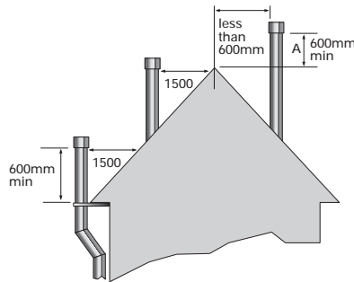
Figure B BS 5440-1 Gas Termination
