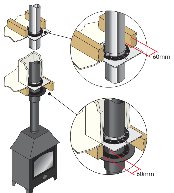
Typical installation of ICS25 through a combustible floor and shaft
