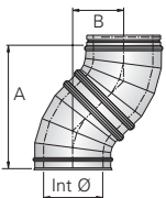
Offsets for Double 45° Bend
